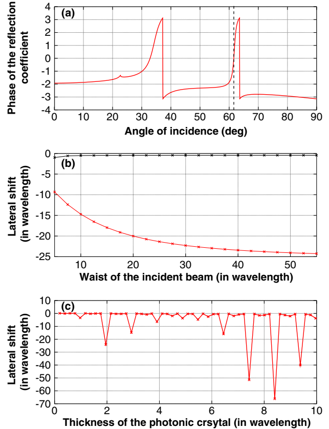
Fig. 2. (Color online) (a) Phase of the reflection coefficient for the 10-period structure considered in Fig. 1, showing that the phase presents a positive derivative characteristic of the negative lateral shift; (b) lateral shift as a function of the waist for an incidence angle of 61.7^\circ corresponding to a swift variation of the phase (red curve at bottom) and for 58^\circ (black curve at top) leading to a smaller shift; (c) lateral shift as a function of the thickness.
