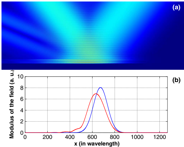
Fig. 3. (Color online) (a) Gaussian beam illuminating a thin slab (seven periods) of a photonic crystal with an incidence angle of 40^\circ and a waist of 89\lambda , (b) profile of the reflected H field showing how it is slightly distorted and shifted toward the left. The field plotted here is the zero-order only. The -1 diffraction order can be seen on the left of the picture—its profile is due partly to the incoming beam and partly to the resonance inside the structure.
